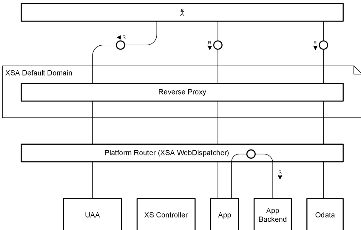
Request Flow with Direct Routing of Internal Requests
