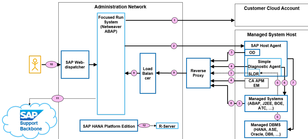
Client/Server Relations in SAP Focused Run 2.0 Technical System Landscape
