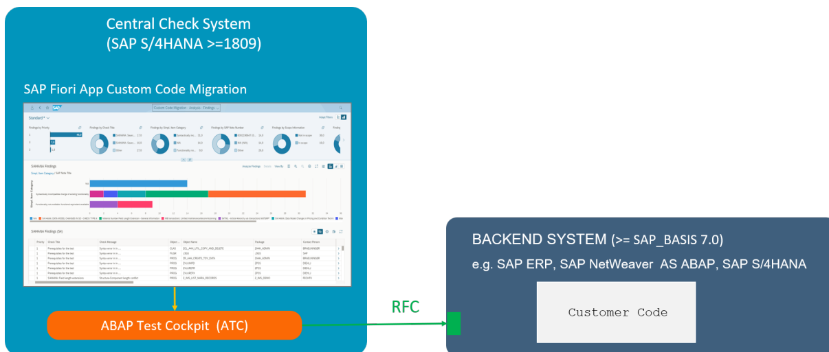
Setup of the remote custom code adaptation of the check results investigated using the Custom Code Migration app
