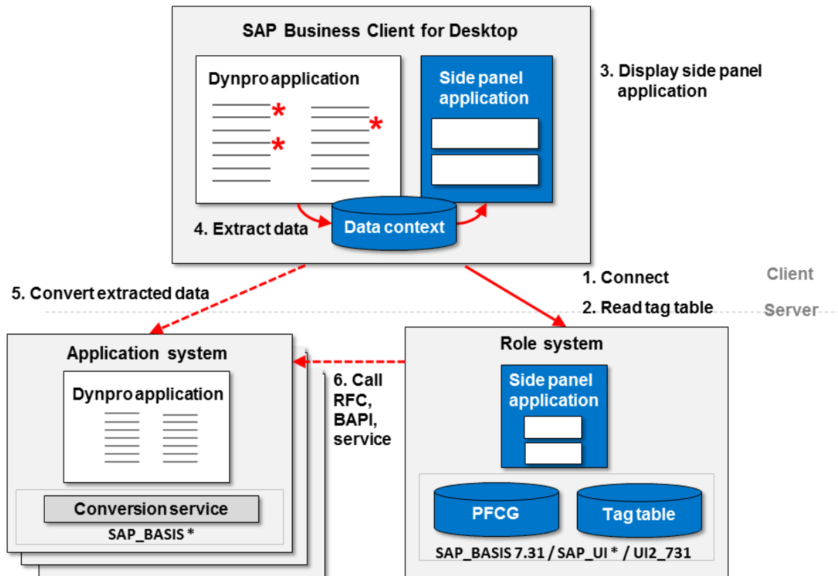
Side Panel Architecture - SAP Business Client Connection
